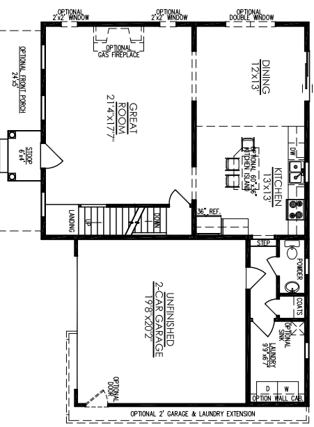
FIRST FLOOR PLAN - A (STANDARD)
