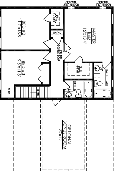
SECOND FLOOR PLAN - A (STANDARD)
