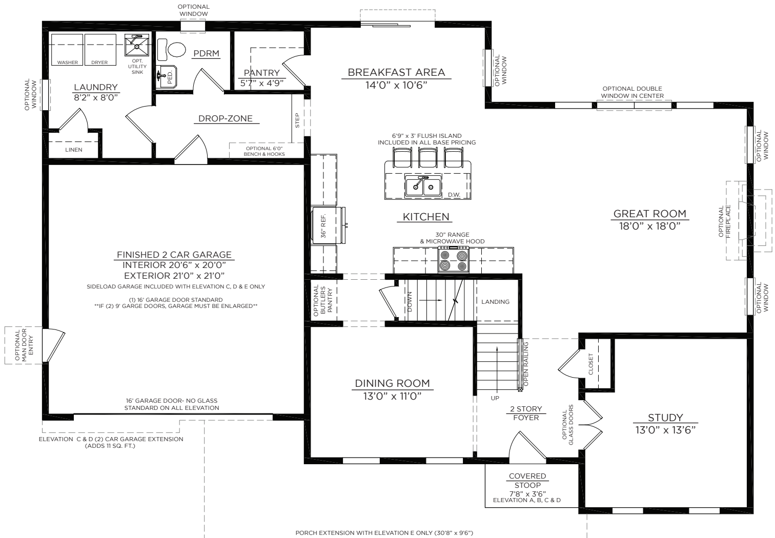
STANDARD FIRST FLOOR PLAN
