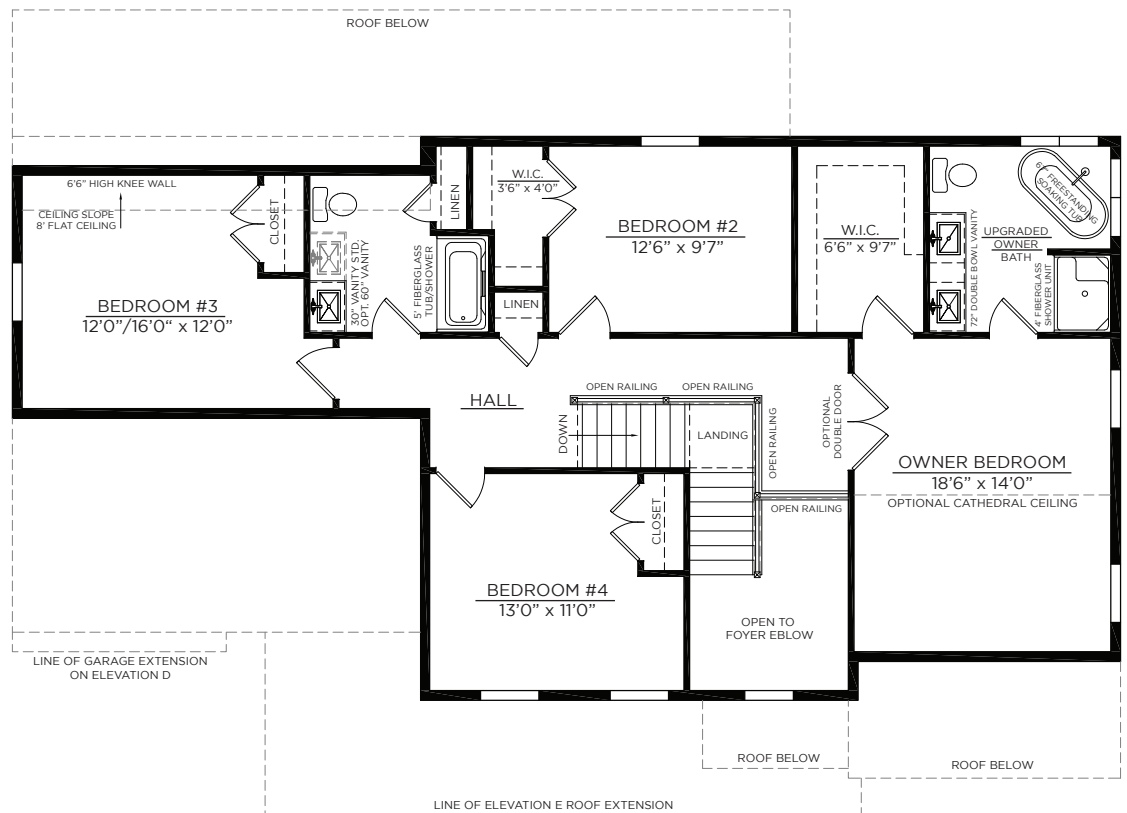
UPGRADED SECOND FLOOR PLAN 4 BEDROOMS, 2 BATHS
