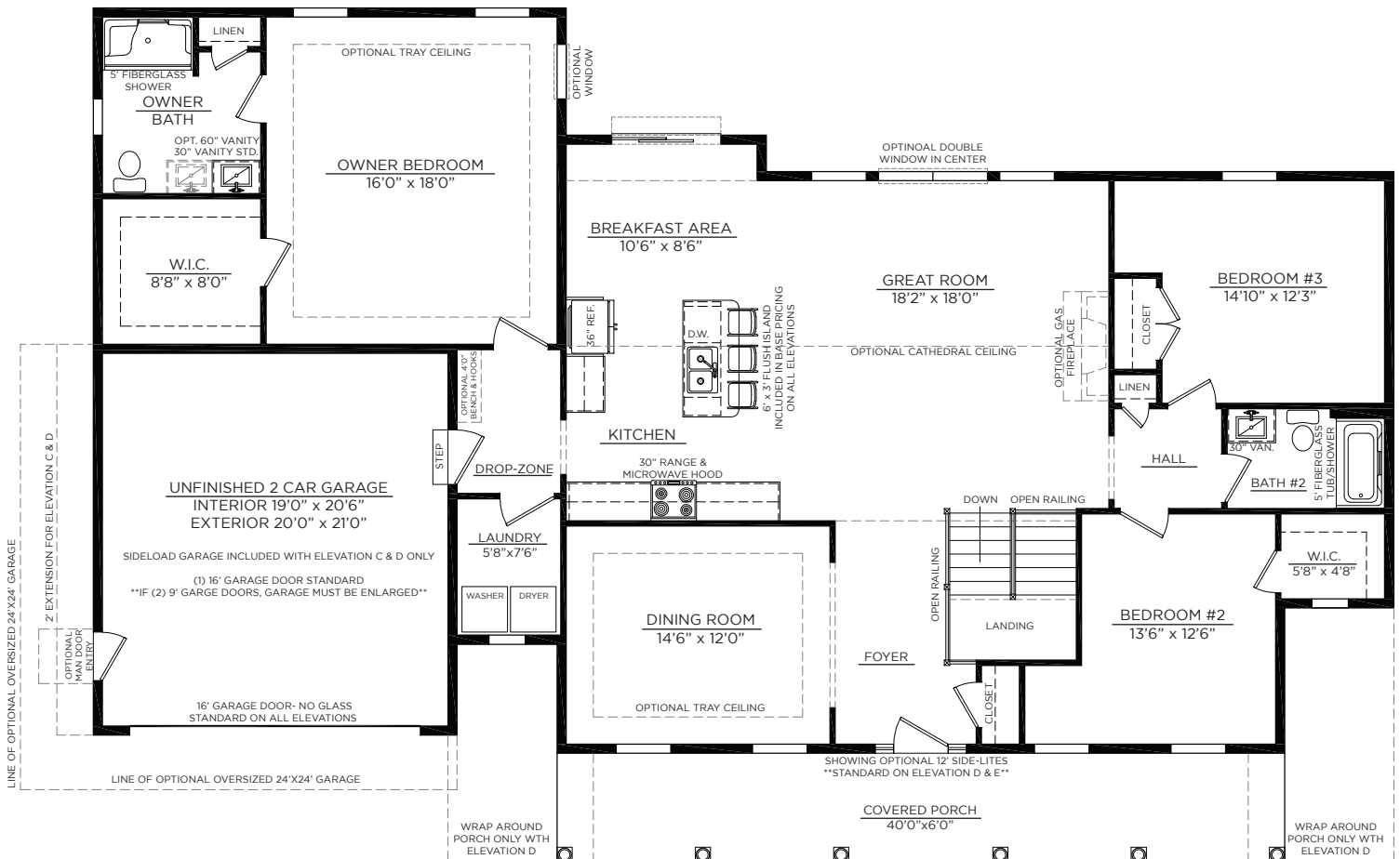
FIRST FLOOR PLAN 3 BEDROOMS, 2 BATHS
