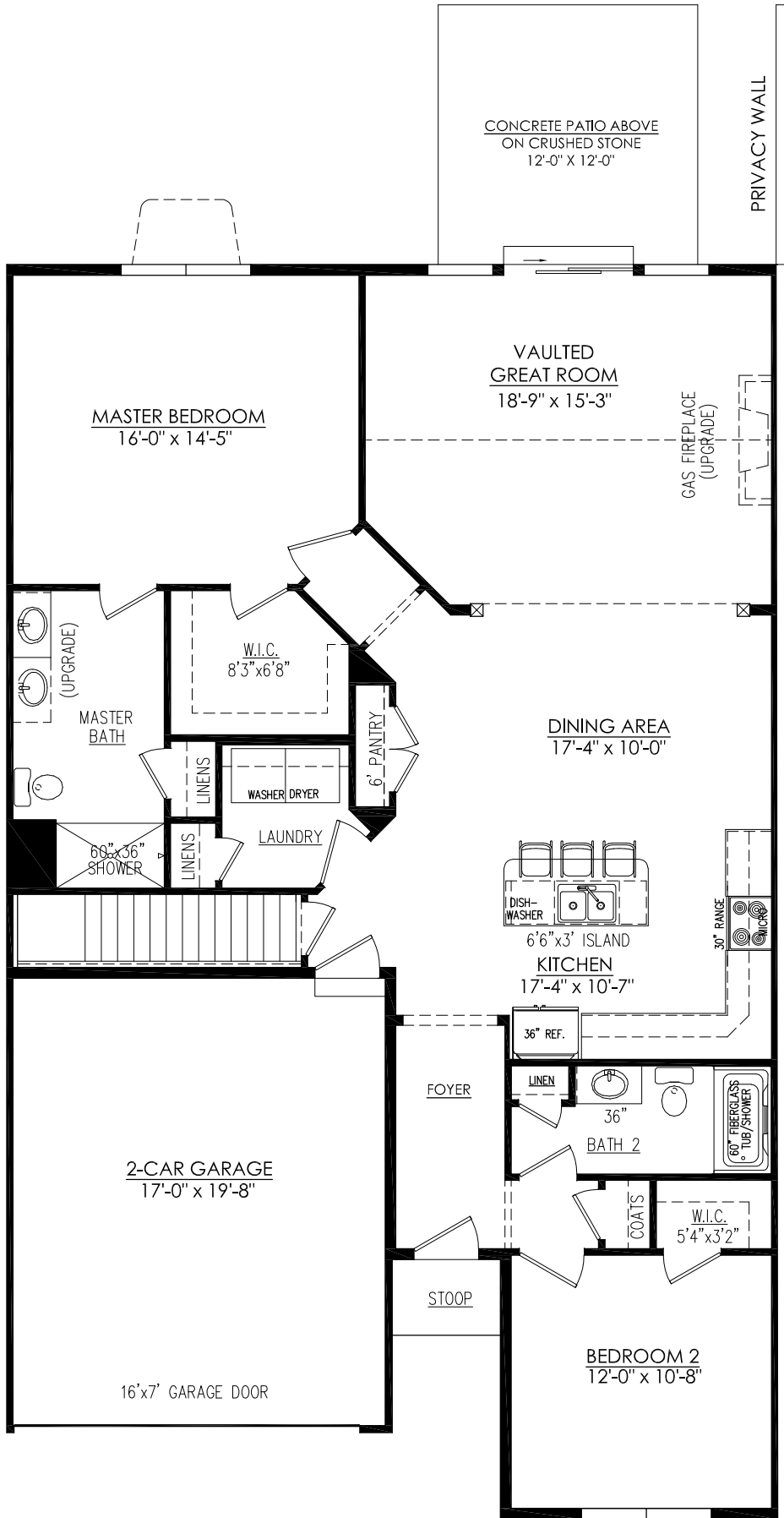
FIRST FLOOR
