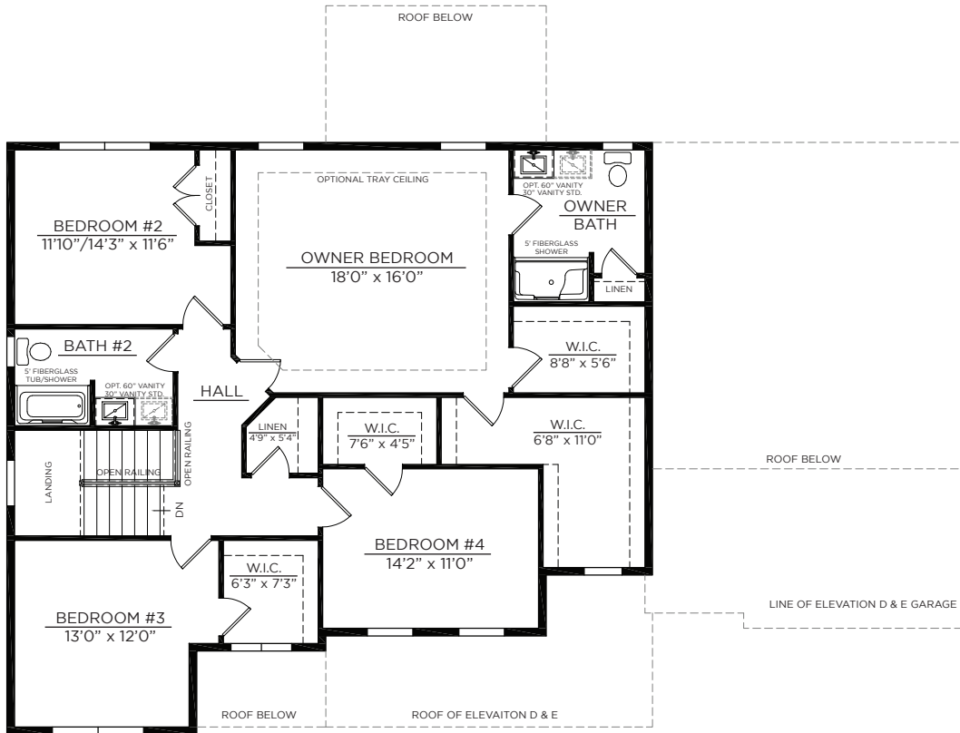
STANDARD SECOND FLOOR PLAN 4 BEDROOMS, 2 BATHS
